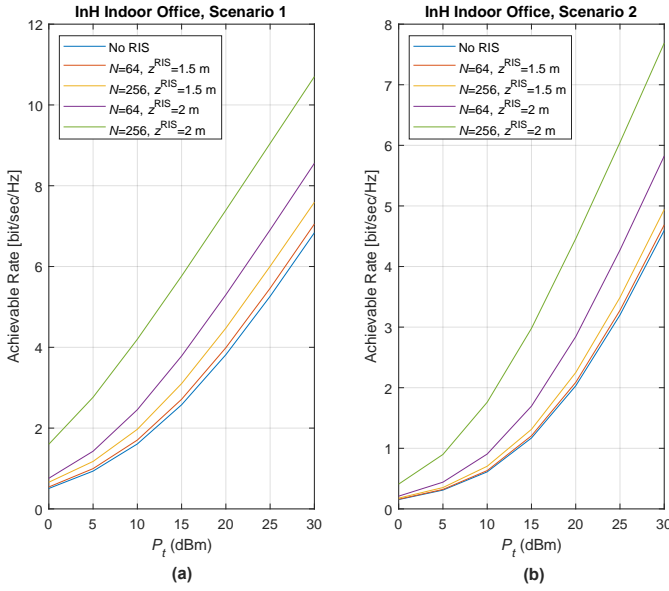
Fig. 5. Achievable rates of RIS-assisted systems for indoors under (a) Scenario 1 and (b) Scenario 2.
